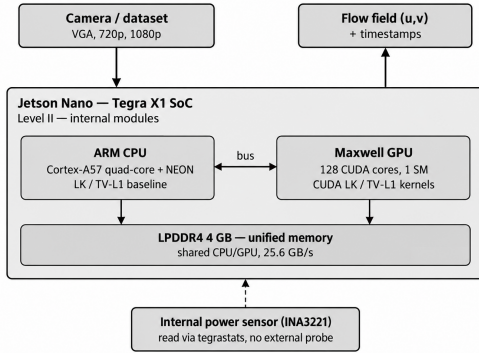
Fig. 3. Level II hardware architecture and data flow for optical flow processing on the Jetson Nano.
