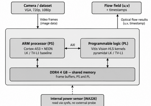
Fig. 2. Level II hardware architecture and data flow for optical flow processing on the Kria KV260.
